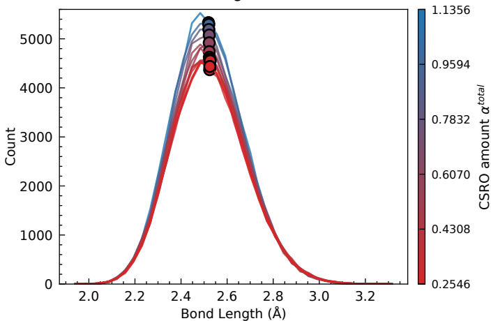
Cr-Co Bond Length Distribution
